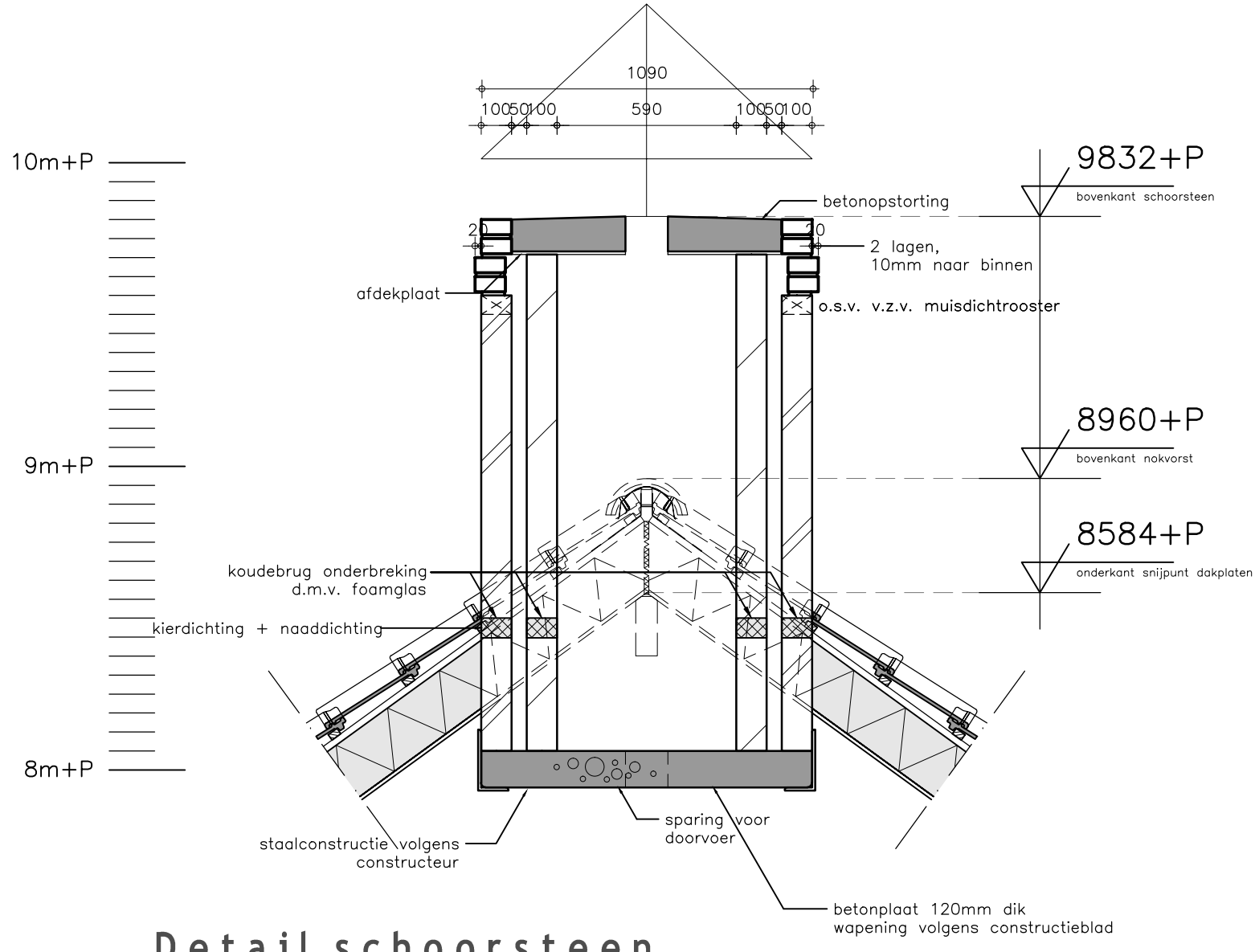
Detail schoorsteen
