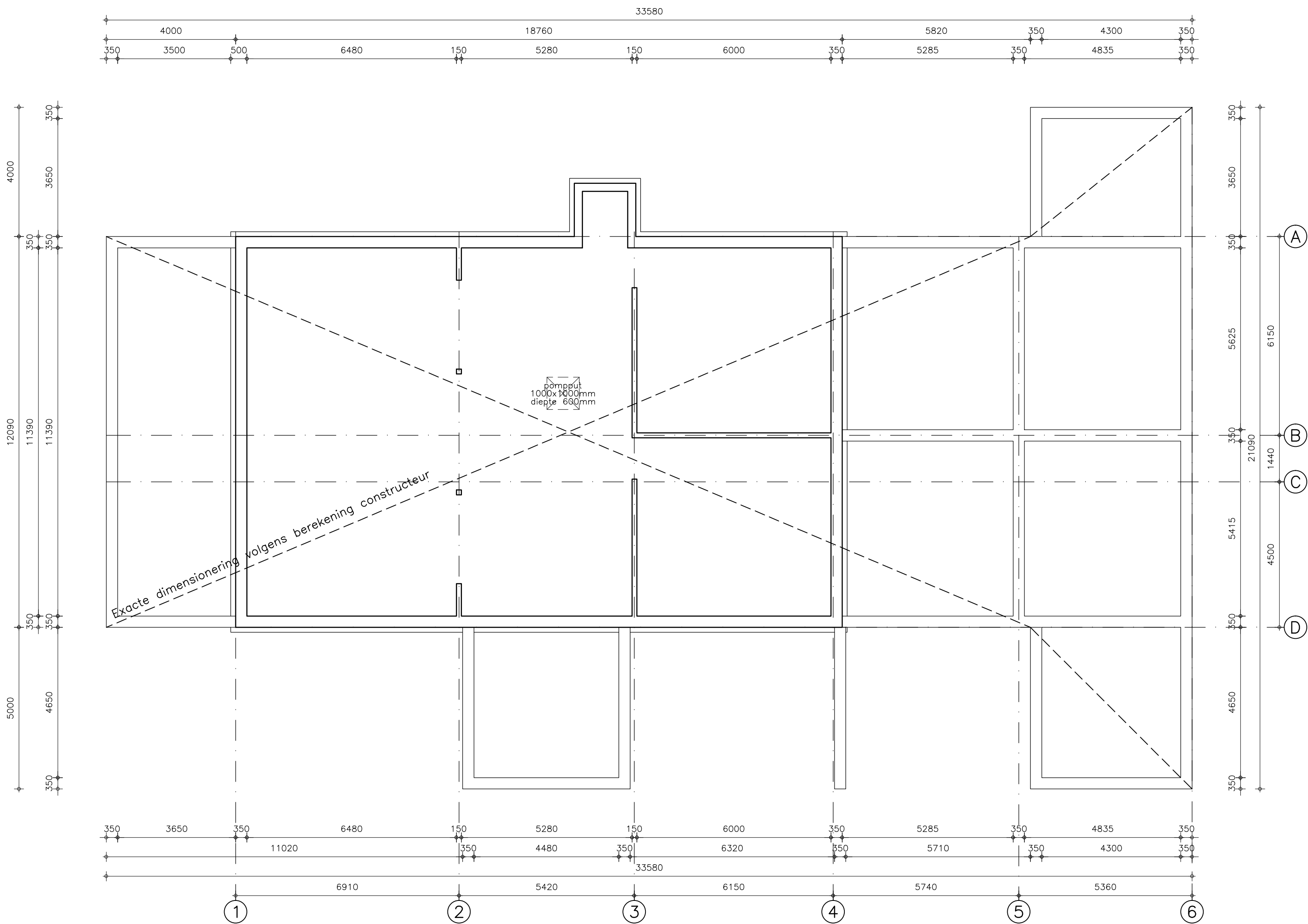
Funderingsplan
