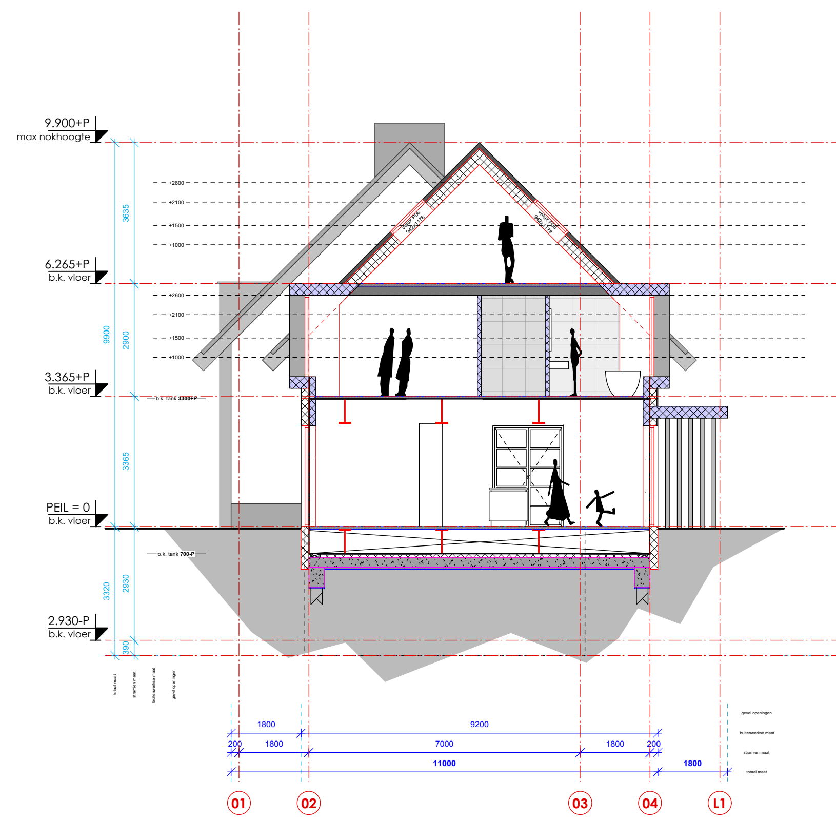
DOORSNED E B B
